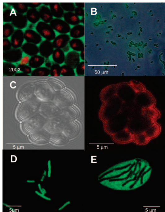
FIGURE 7. (A) Lipid-coated CdSe nanocrystals (red) localize at the cell surface during CDA and are then internalized by yeast cells within 24 h. Green fluorescence is due to labeled lipid, d1C_6PC-NBD , localized at the cell surface. (B) E. coli cells that have been genetically modified in situ by plasmid localization during CDA show GFP expression in response to the analyte arabinose. (C) DIC and confocal fluorescence image of BR (labeled with Alexa Fluor 594) organized around yeast cells in a lipid-templated silica film formed by CDA with added BR-containing liposomes. Fluorescent pH probe shows the pH gradient that develops during CDA for (D) E. coli and (E) B. subtilis .
