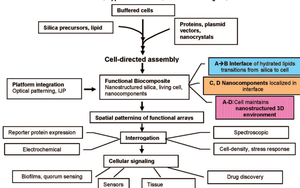
Scheme 1. CDA Process, Applications of CDA, and the Resulting Bio/Nano Interface a
